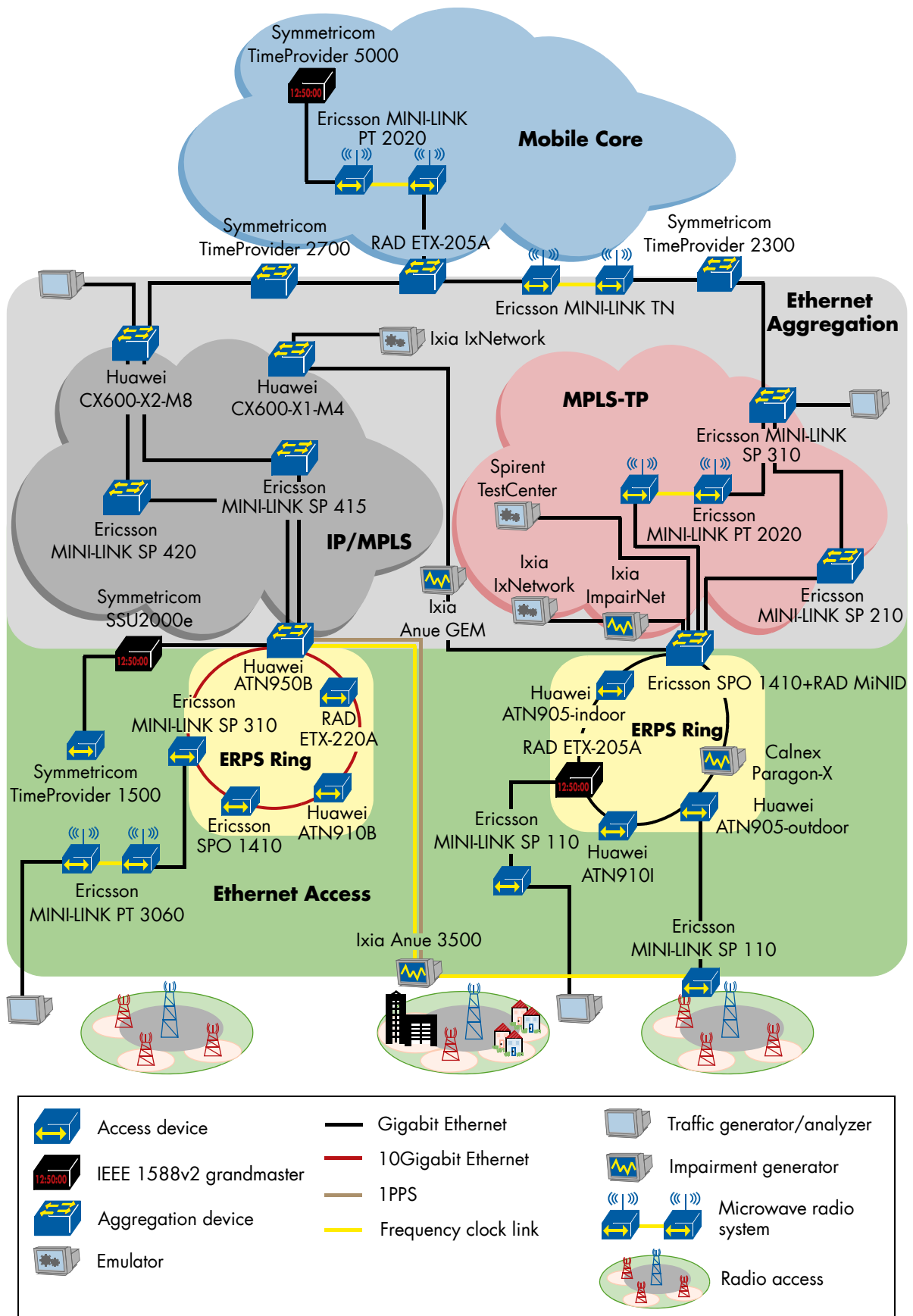
SHOWCASE NETWORK TOPOLOGY
