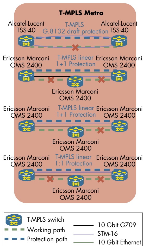
Figure 15: T-MPLS protection
