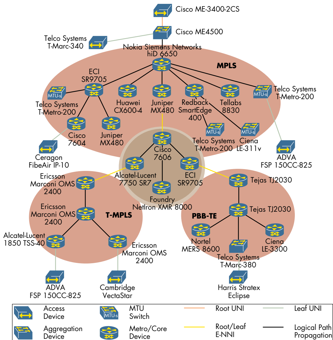
Figure 1: E-Tree logical connections
