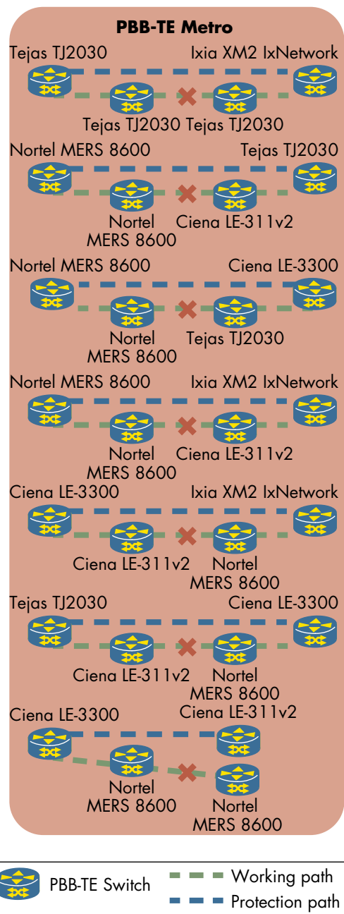
Figure 14: PBB-TE protection results
